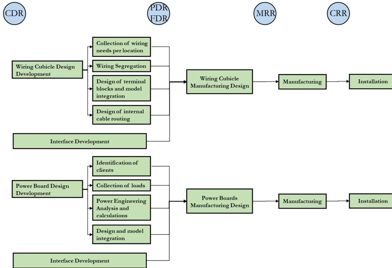
Figure 1 Design Development for wiring cubicles, electrical sub-distribution panels. These components are currently in post-installation or in installation phase.
